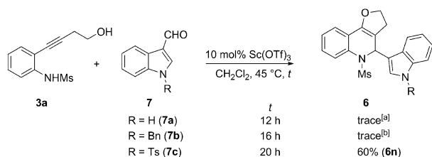
Scheme 2. Bicyclization reaction of the o -alkynylaniline 3a with indole-3-carbaldehyde. [a] 7a was recovered in 35% as determined by 1 H NMR analysis. [b] 7b was recovered in 84% as determined by 1 H NMR analysis.
